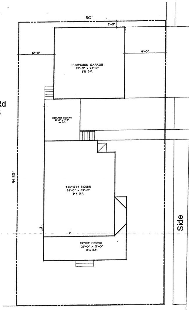
Birch Swamp Rd SITE PLAN - PROPOSED SCALE: 1/2"
